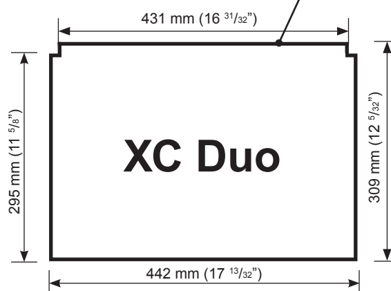
Measurements of the stove installation cut-out.
