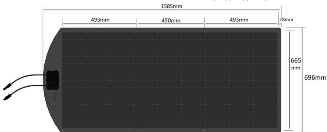
UNISUN 150.12MS
