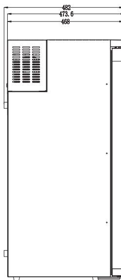
LR90L (713507)
