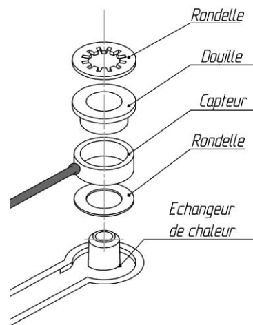
Fig.8 – Capteur de surchauffe (thermocouple)
