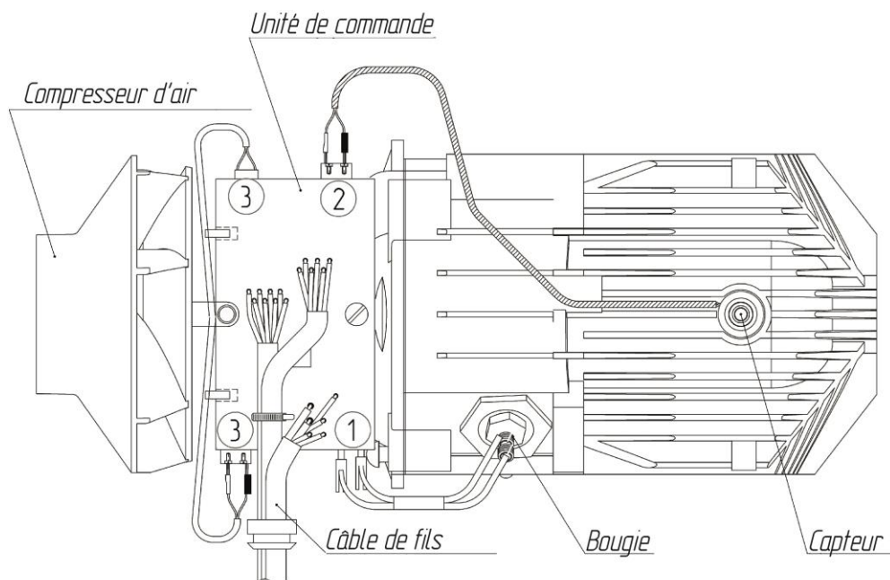
Figure 2 - Élément chauffant
